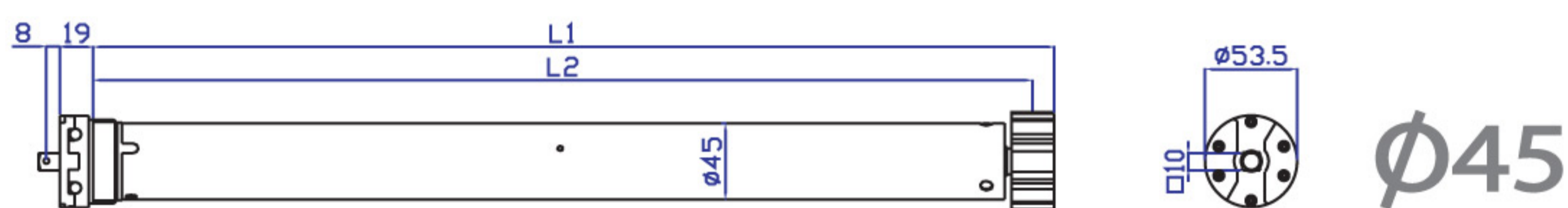
Dimension drawing
