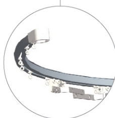
Curved Track Minimum Radius of curved track 250cm Minimum Curtain Case of curved track 200mm
